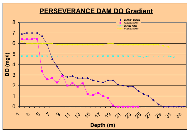
Figure 8. Dissolved oxygen gradient before and after a WEARS Close Coupled SMDI-5 system was installed at Perseverance Dam.
